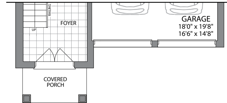
PARTIAL MAIN LEVEL - ELEV. B
