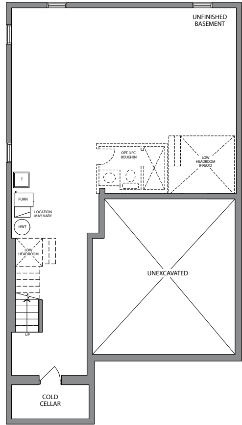
LOWER LEVEL - ELEV. A
