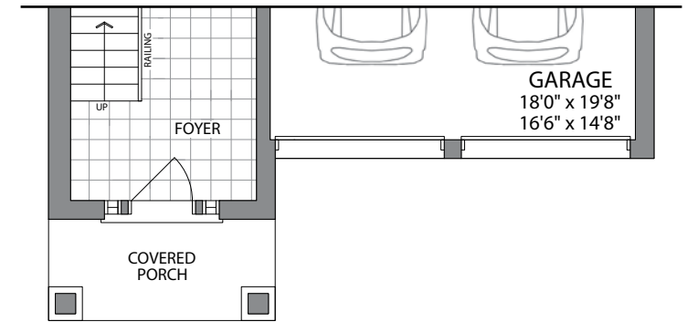
PARTIAL MAIN LEVEL - ELEV. C
